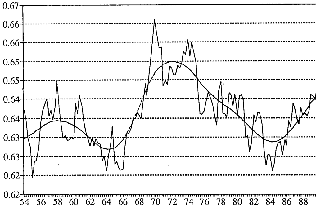
Labor's Share of GNP: Measure 2
