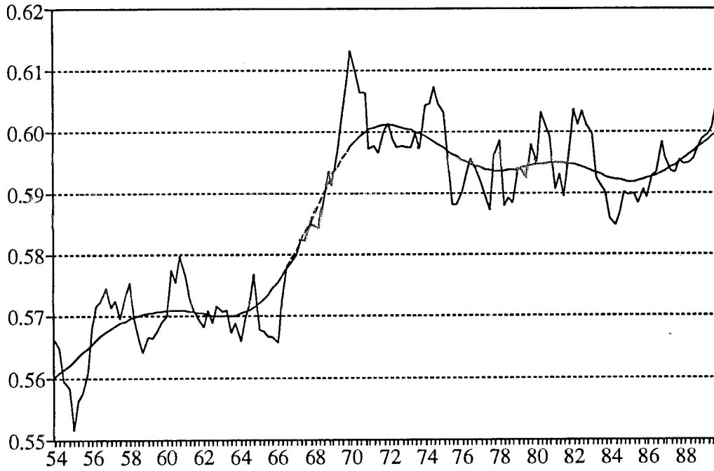
Figure 1 Labor's Share of GNP: Measure 1
